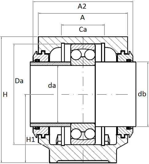
Labyrinth seal
