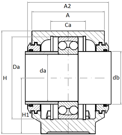
Labyrinth seal
